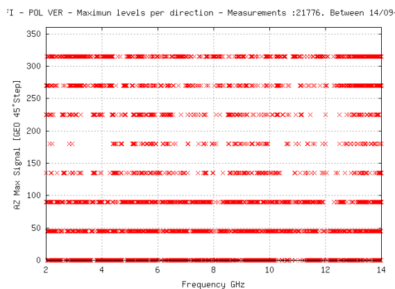
Fig. 5 Azimuth direction vs. observed spectrum. The amount of detected events is correlated with the directions in which urbanized areas are located. The Southern direction points to a rural area and less events have shown up.
